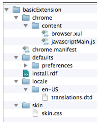
Fig. 2. Typical structure of a Firefox browser extension
