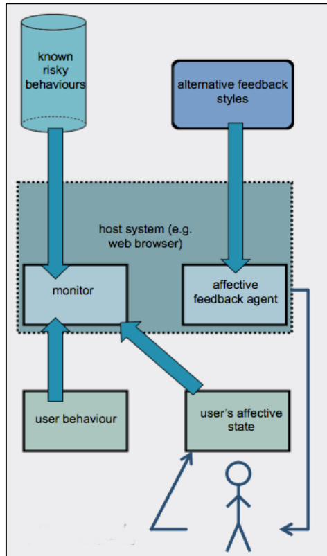
Fig. 1. - Overview of system architecture
