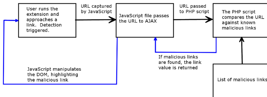
Fig. 3. Overview of the Link Detector extension
