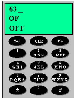
Hybrid Dictionary-based
