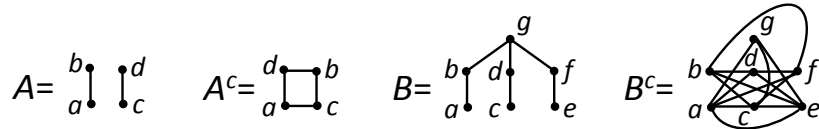
FIGURE 9. Graphs A and B and their complements A^c and B^c .
