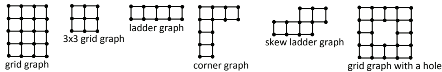
FIGURE 10. Induced subgraphs of a grid graph.
