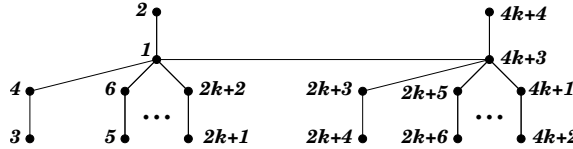
FIGURE 6. The labeling of DC(P_2) .
