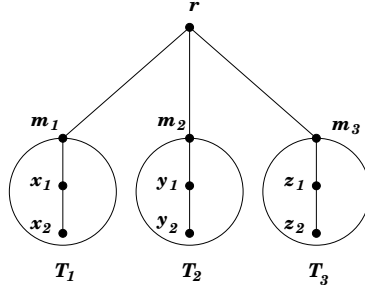
FIGURE 3. The structure of components in T \setminus v which are not good.
